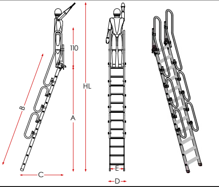
Poggia scala. Ladder rests
