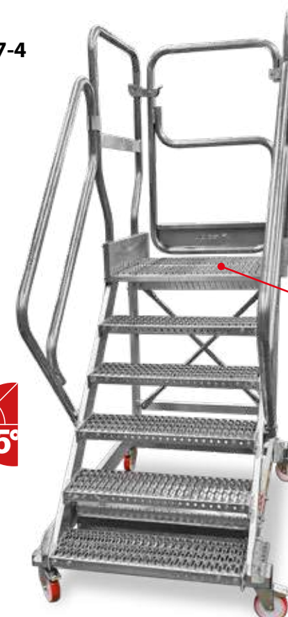
Scala a castello con spondina ribaltabile e gradini e passerella con griglia antiscivolo. Warehouse ladder with foldable handrail and grating steps and walkway with non-slip grid.
